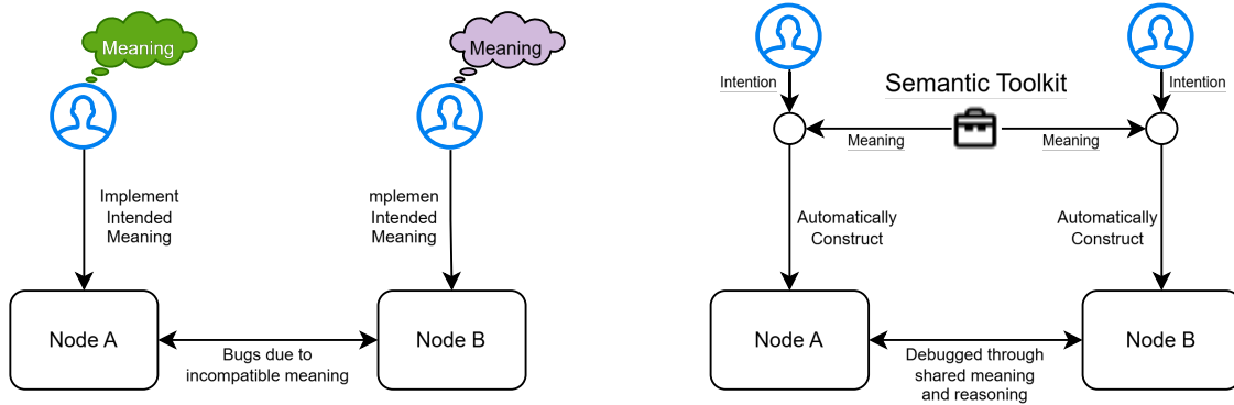
Figure 16: Eliminating bugs within and between systems using semantic toolkit
