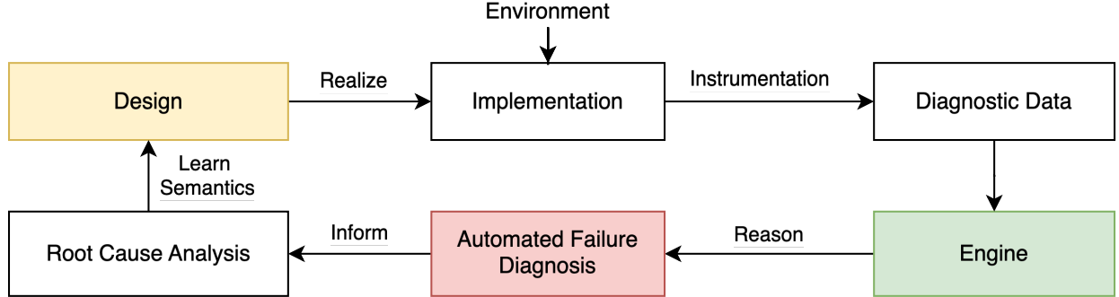
Figure 6: Ideal learning loop by reasoning about execution using design meaning
