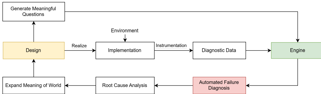
Figure 8: Ideal learning loop by reasoning about execution using design meaning
