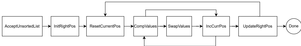
Figure 1: Bubble Sort Behaviors and Narratives
