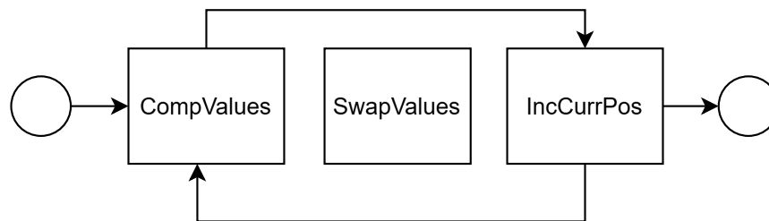
Figure 2: Complete Bubble Sort Pass
