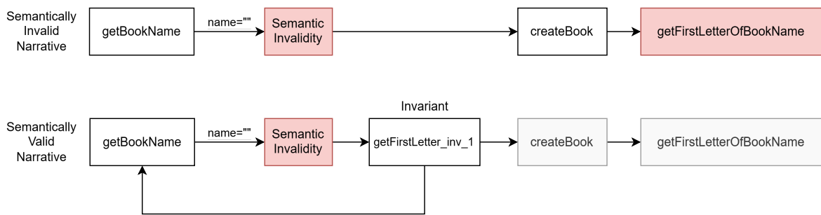
Figure 5: Semantically valid and invalid narratives.
