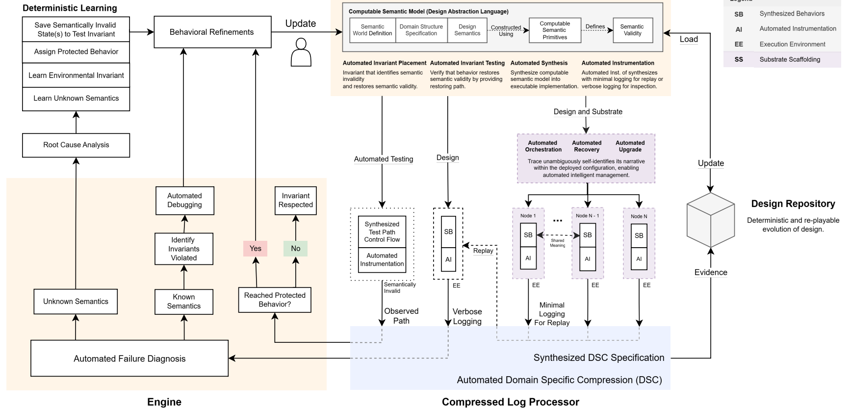
Figure 7: The Design Learning Platform
