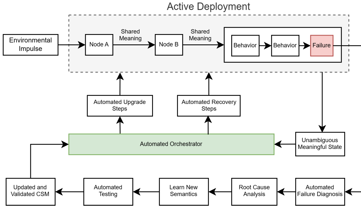
Figure 9: Automated Failure Response
