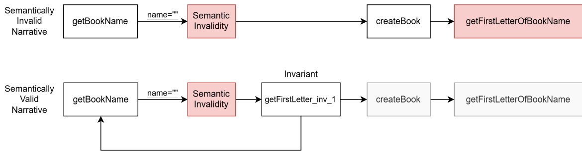
Figure 5: Semantically valid and invalid narratives.
