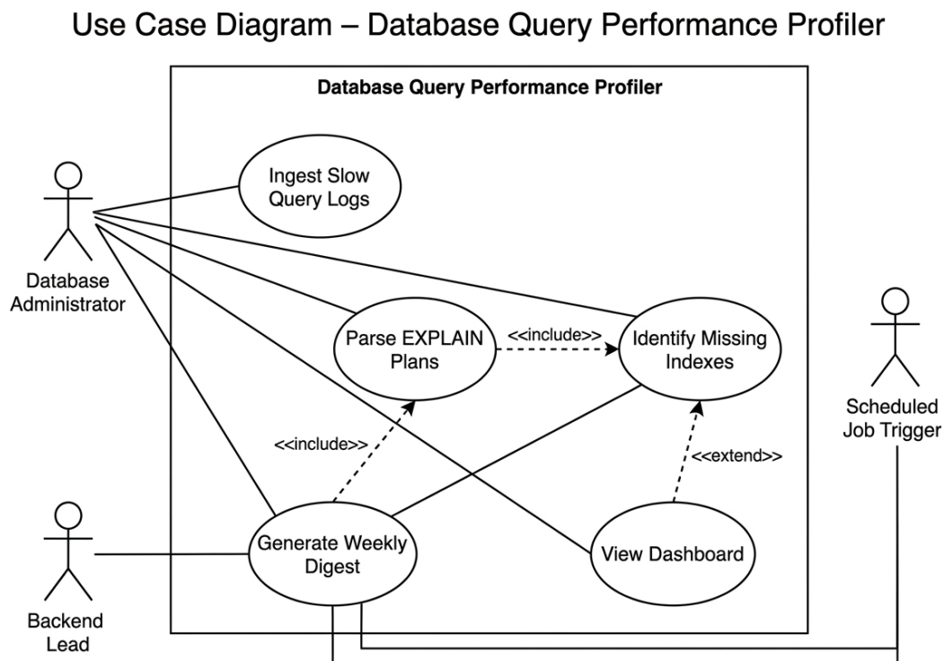
Figure 1 – Use-Case Diagram (draw.io)
