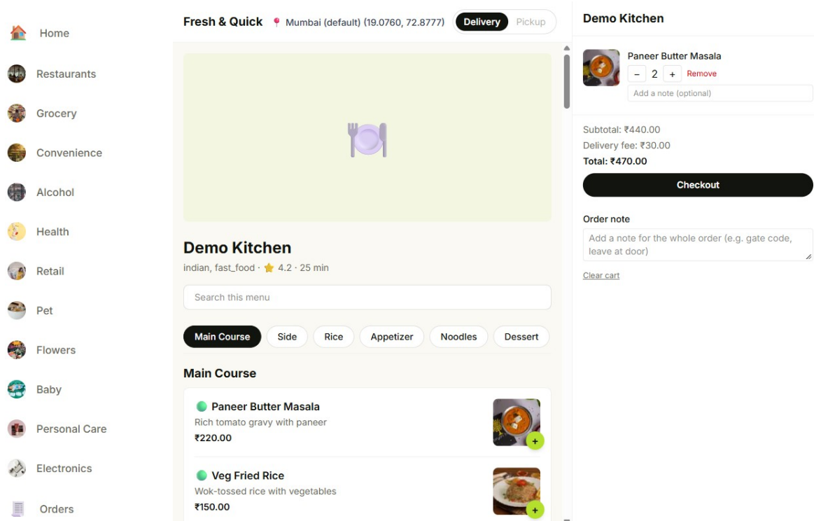
Figure 3.2 — A restaurant's menu page, showing items grouped by category with an Add (+) button on each dish, and the persistent cart panel on the right once an item has been added.
