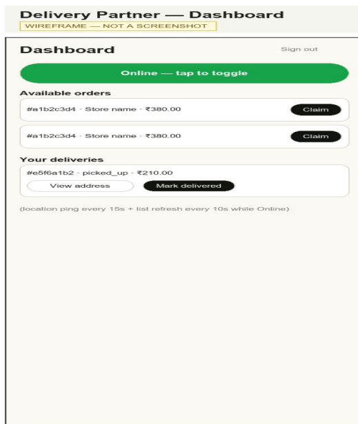
Wireframe — Delivery Partner dashboard (online toggle, available orders with Claim, your deliveries with status-advance and View address) (illustrative wireframe from v2.0; real screenshot not yet captured).
