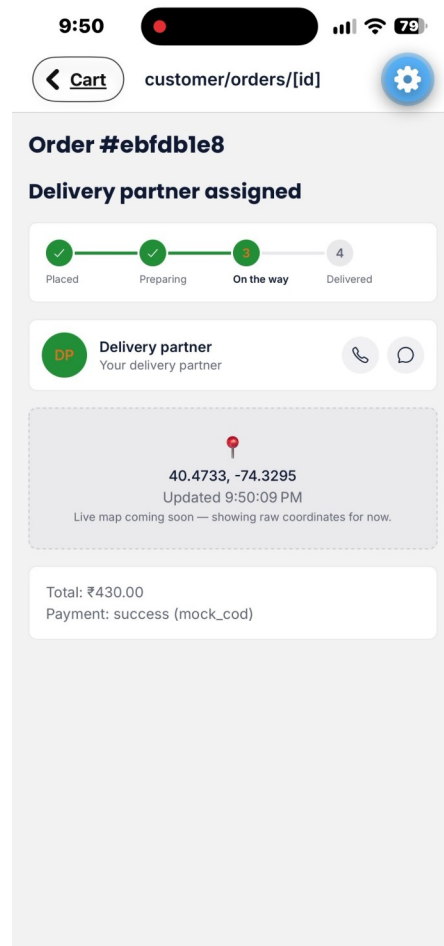
Screenshot — Order Tracking: status stepper, courier card, and coordinate readout.
