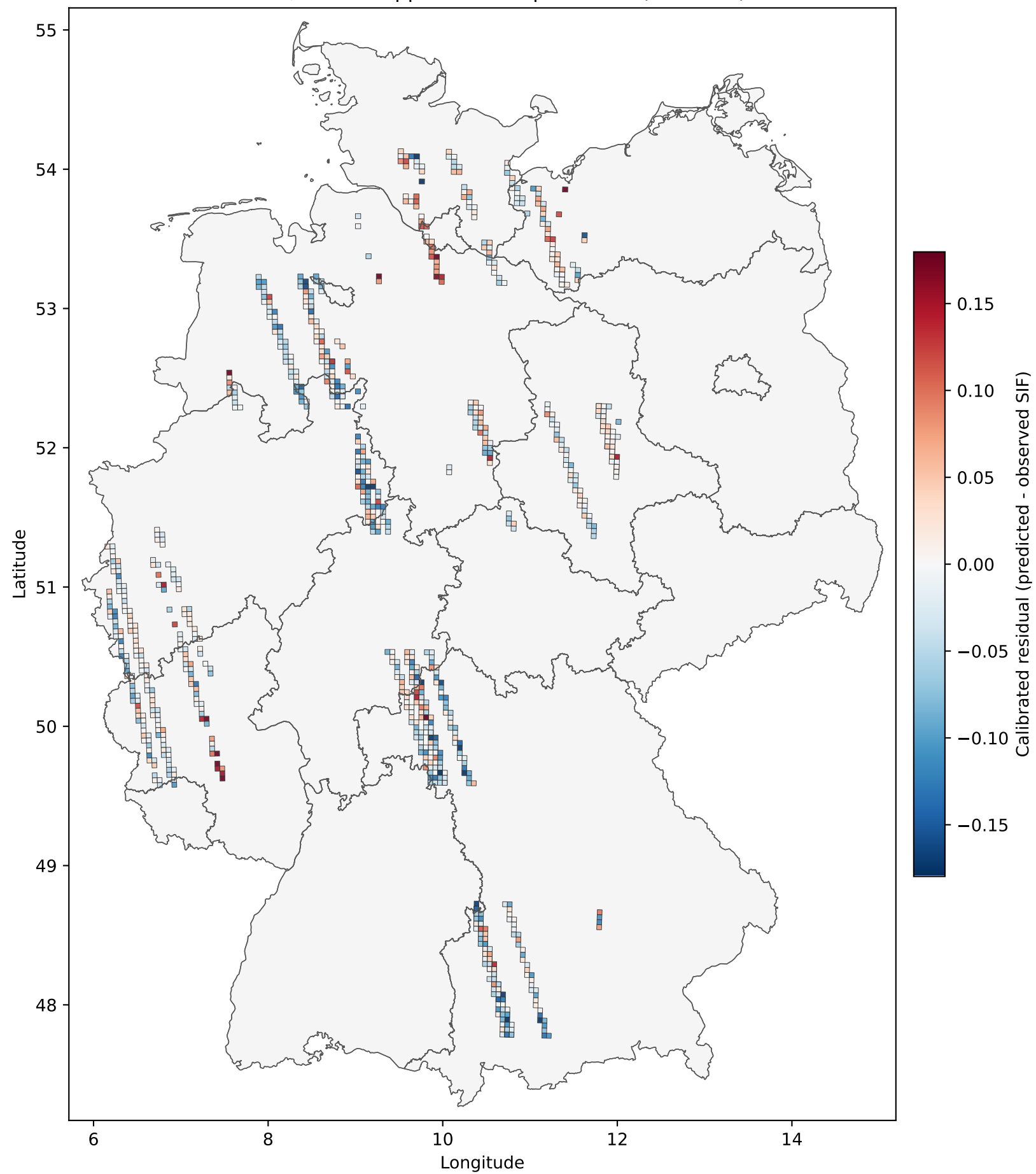
Spatial distribution of calibrated 4 km test residuals over Germany N=931; colour clipped at 98th percentile ( \pm 0.180 )
