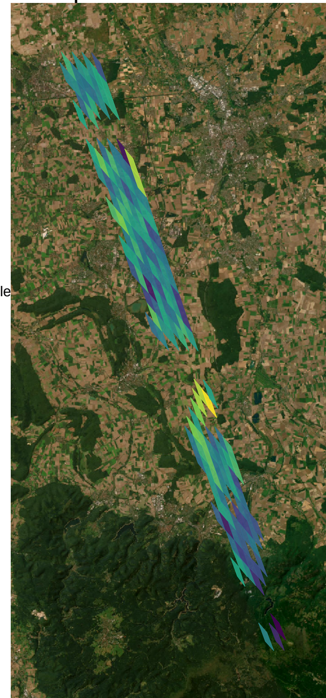
SIF footprint value
