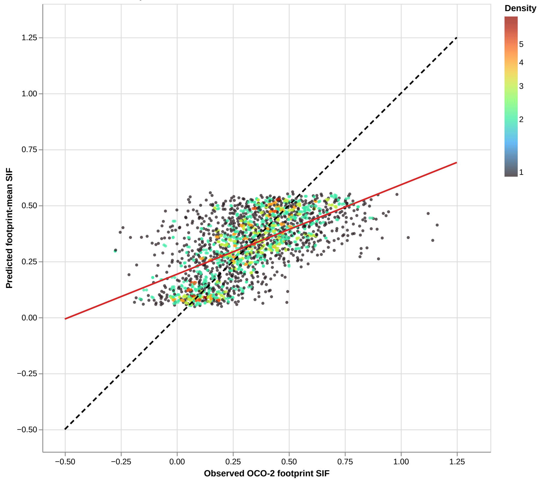
External Native-Footprint SIF Evaluation: Observed vs. Predicted SIF, RMSE=0.1701, R2=0.373
