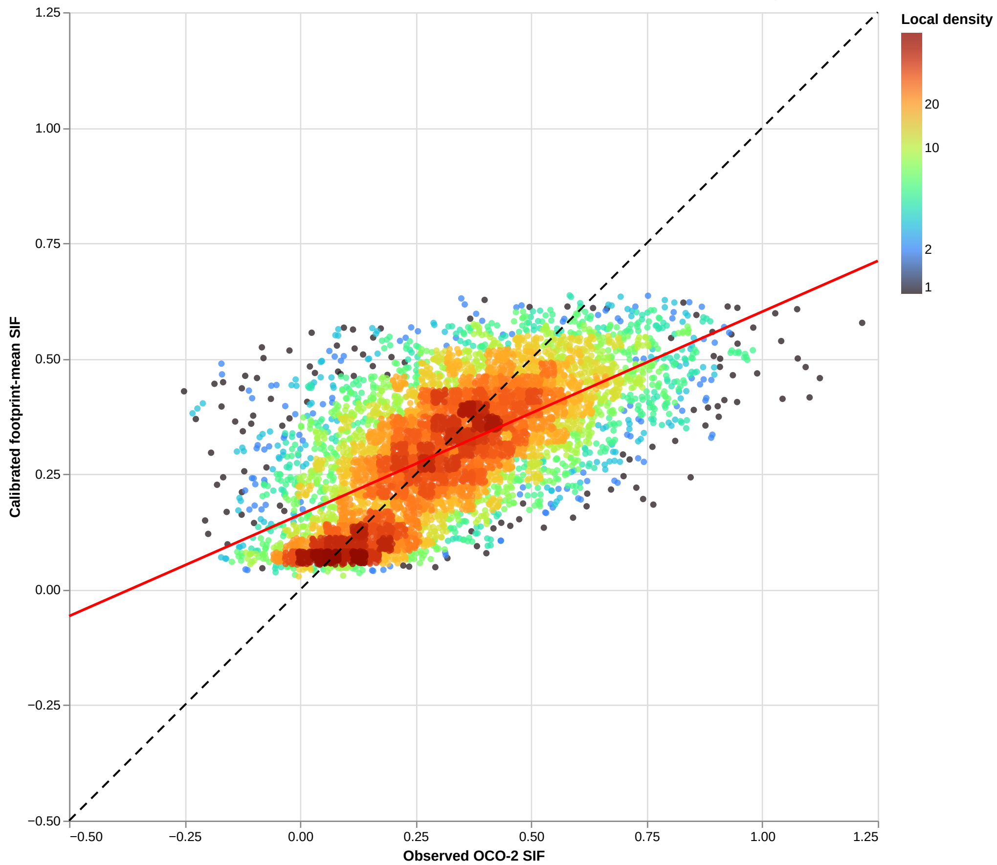
MultiSIF-Sen2: Observed vs. Predicted SIF, Test RMSE=0.1603, R2=0.418, slope=0.439
