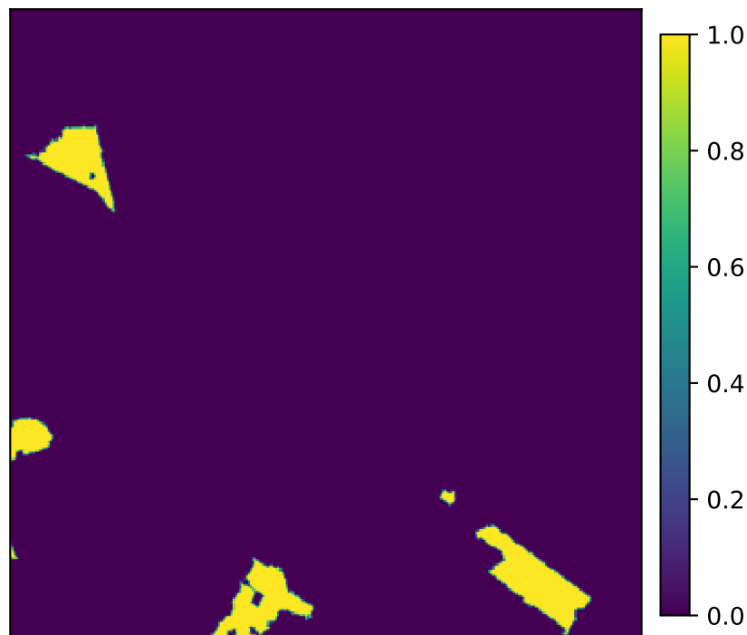
13: woody_fraction valid=1.000
