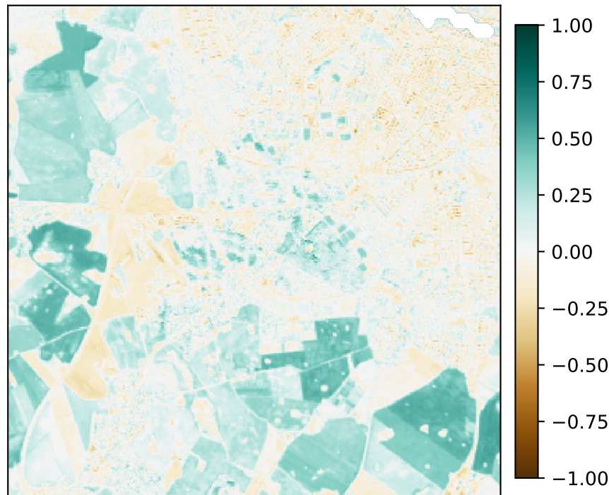
4: ndre valid=0.995
