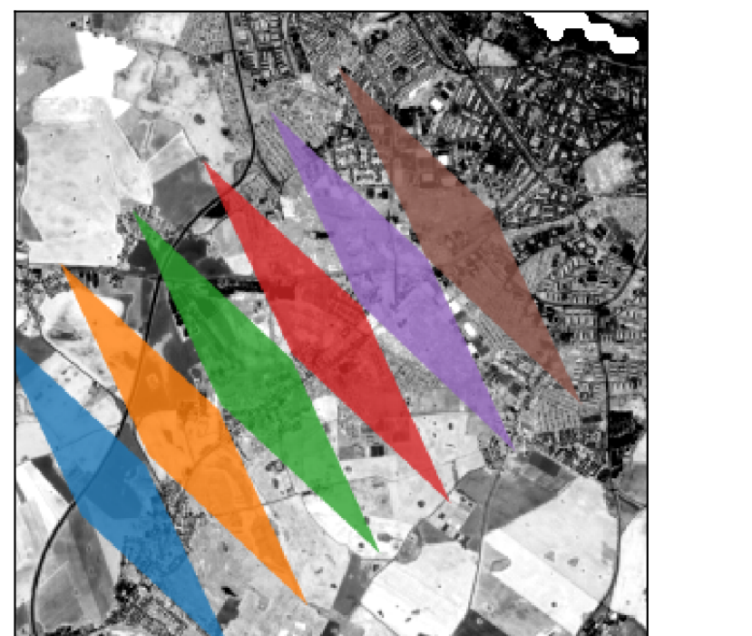
SIF masks over NDVI
