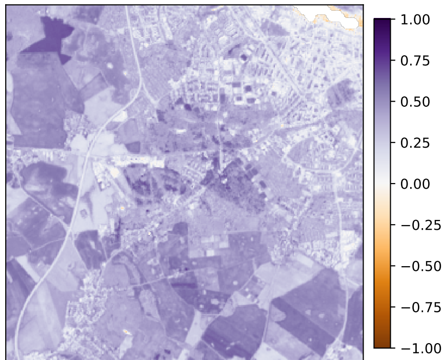
8: winter_wheat_fraction valid=1.000
