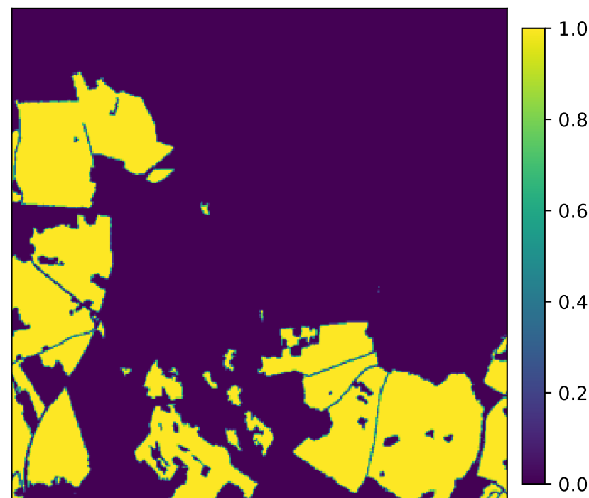
15: active_crop_fraction valid=1.000
