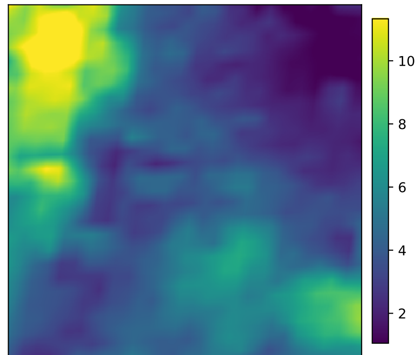
11: maize_fraction valid=1.000
