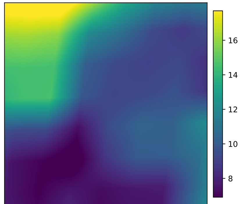
10: winter_rye_fraction valid=1.000
