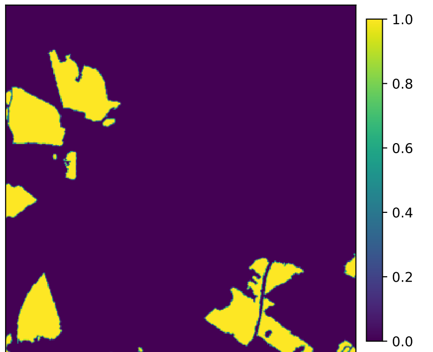
12: grass_forage_fraction valid=1.000
