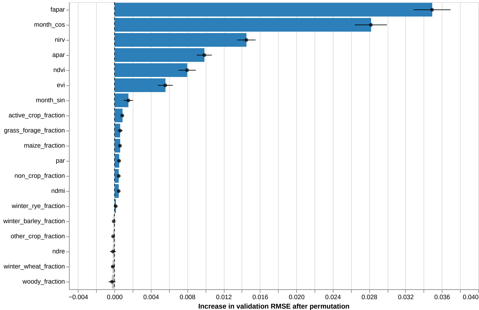
Validation channel permutation importance (3 repeats)
