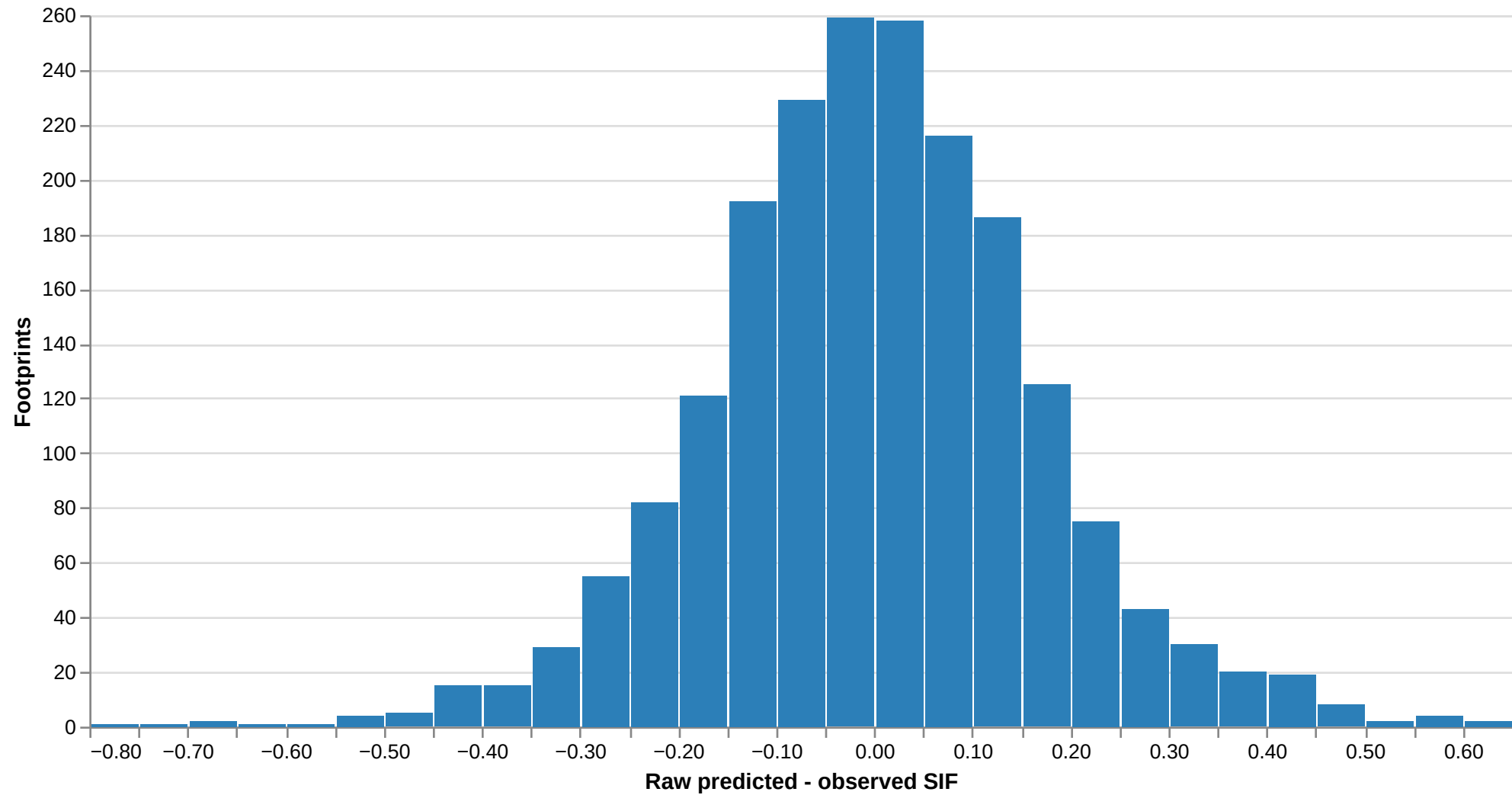
External Native-Footprint SIF Evaluation: Residual Distribution
