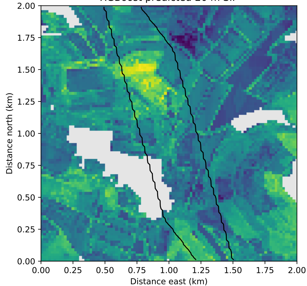
XGBoost predicted 20 m SIF
