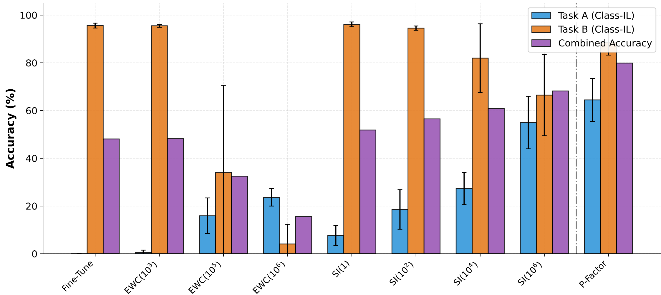
Gradient-Based Baselines vs. P-Factor (Split-MNIST, Epoch 3)
