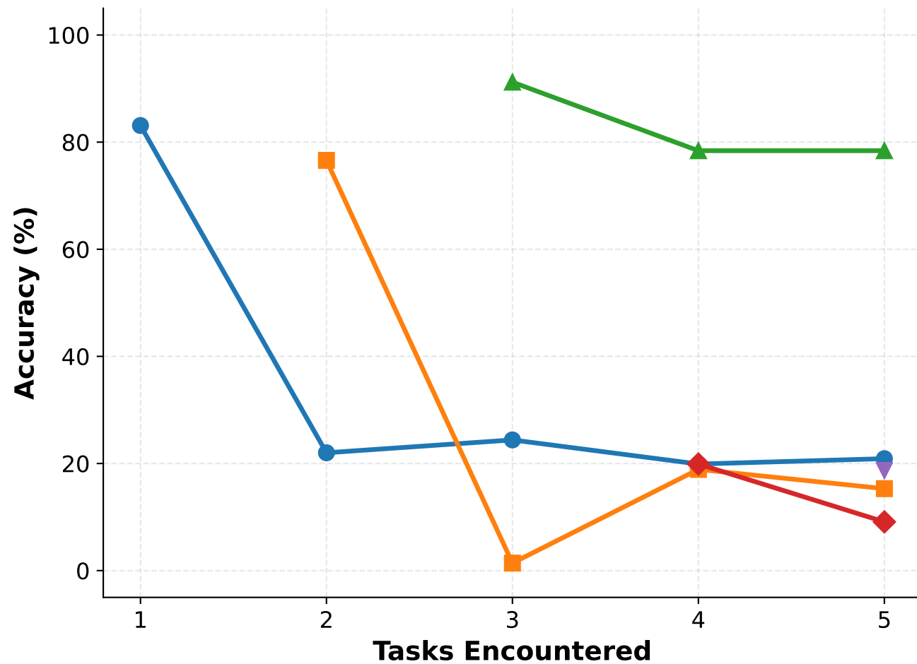
P-Factor Class-IL Trajectory
