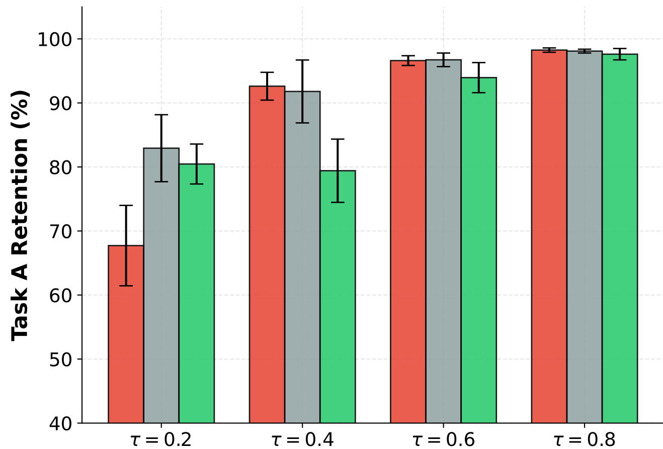
Task-IL Performance
