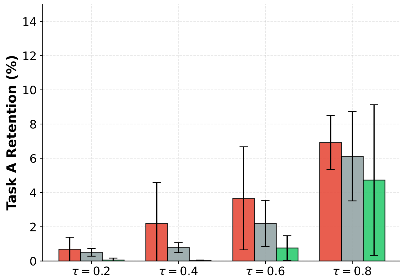
Class-IL Performance
