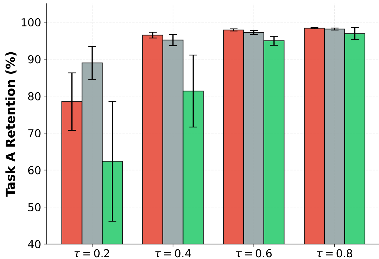
Task-IL Performance
