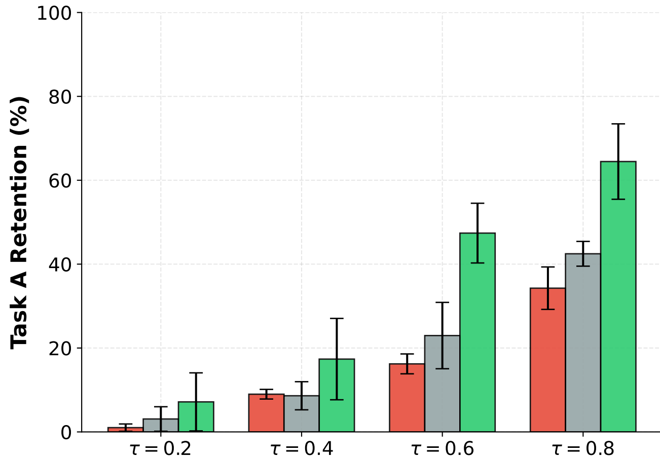
Class-IL Performance
