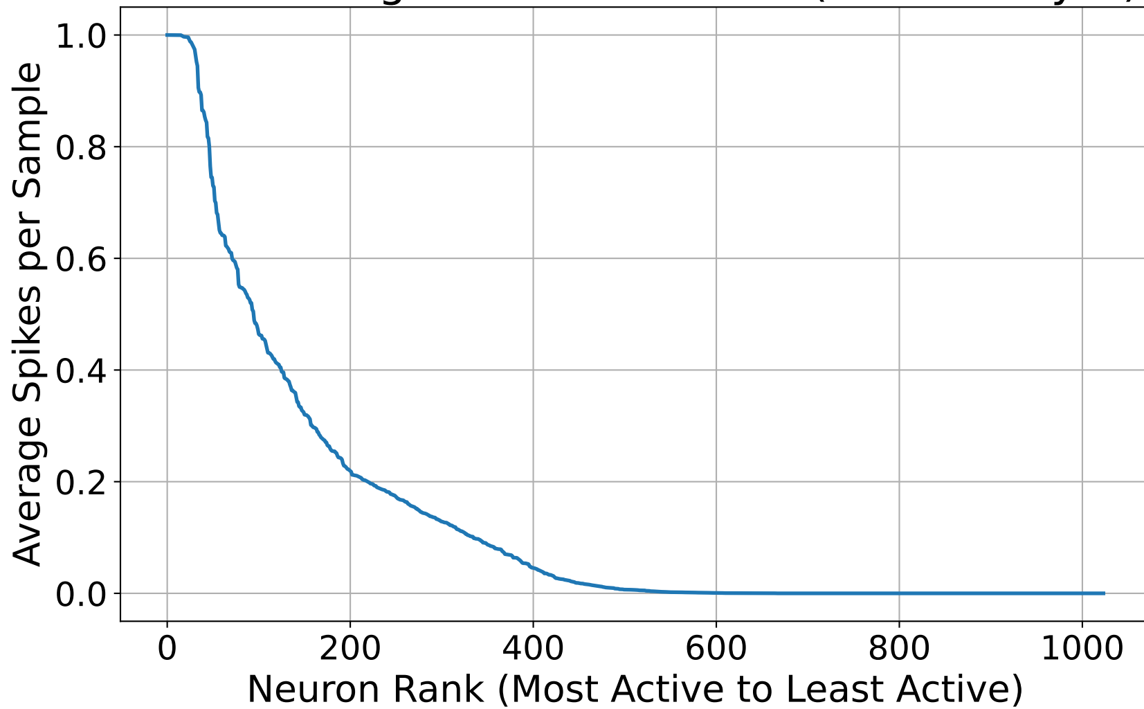
Task A Firing-Rate Distribution (Hidden Layer)
