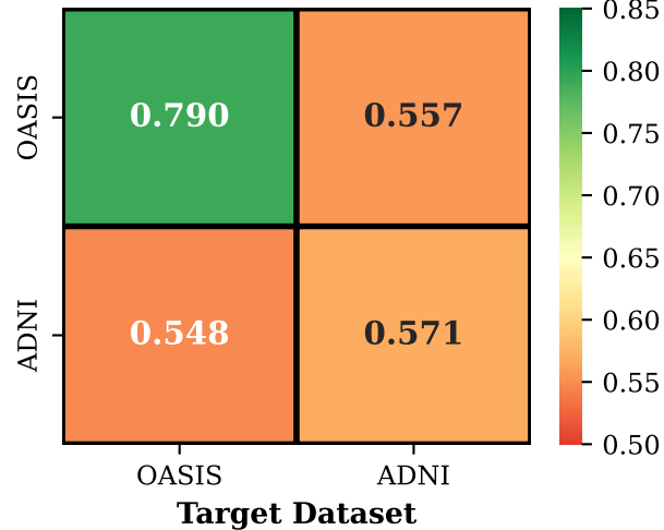
Attention Fusion
