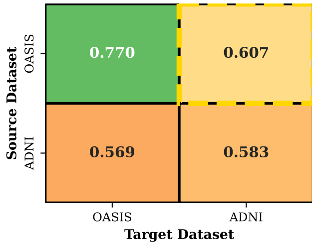
MRI-Only
