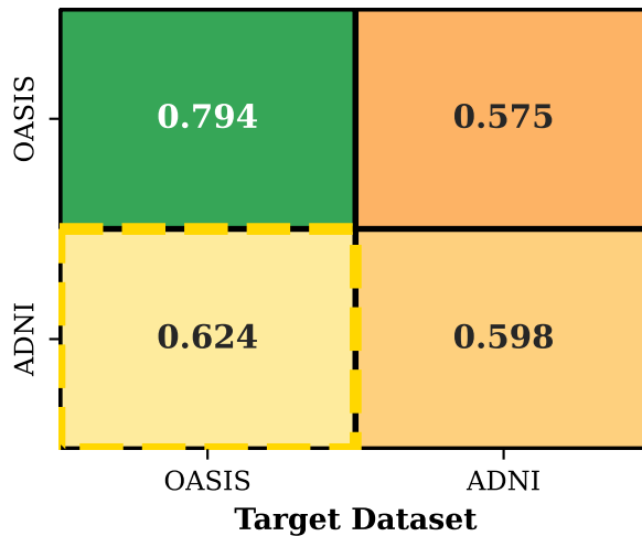
Late Fusion
