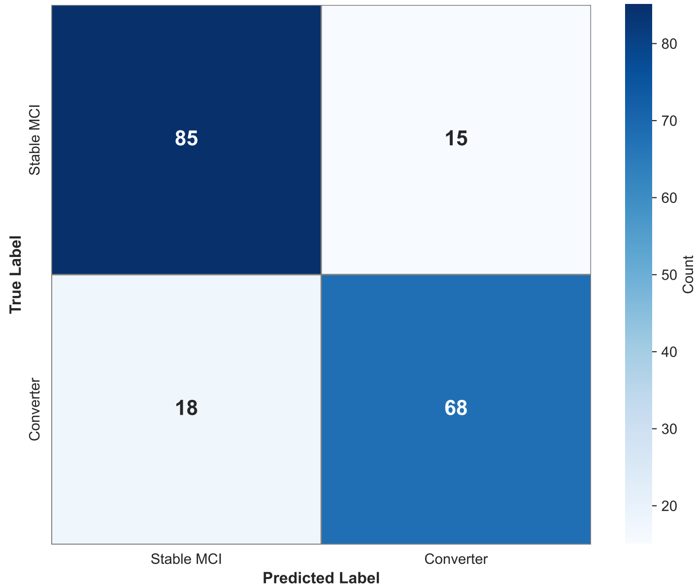
Confusion Matrix: MCI Progression Prediction (Longitudinal Fusion Model)
