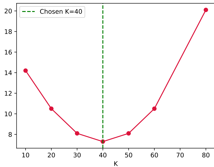
Downstream LR RMSE
