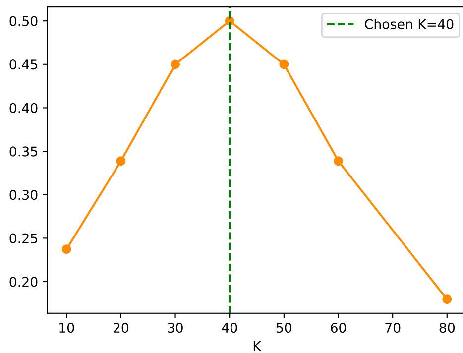
Silhouette Score
