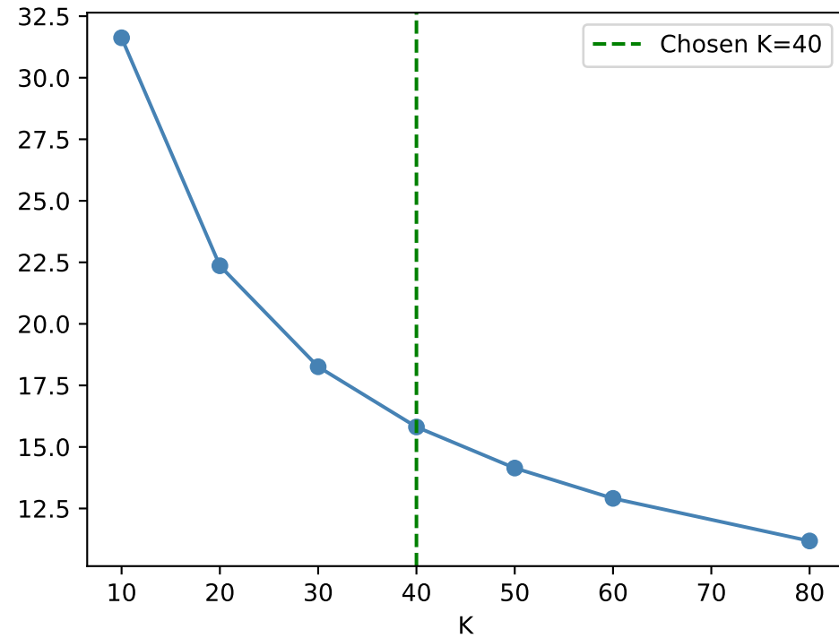
Inertia Elbow
