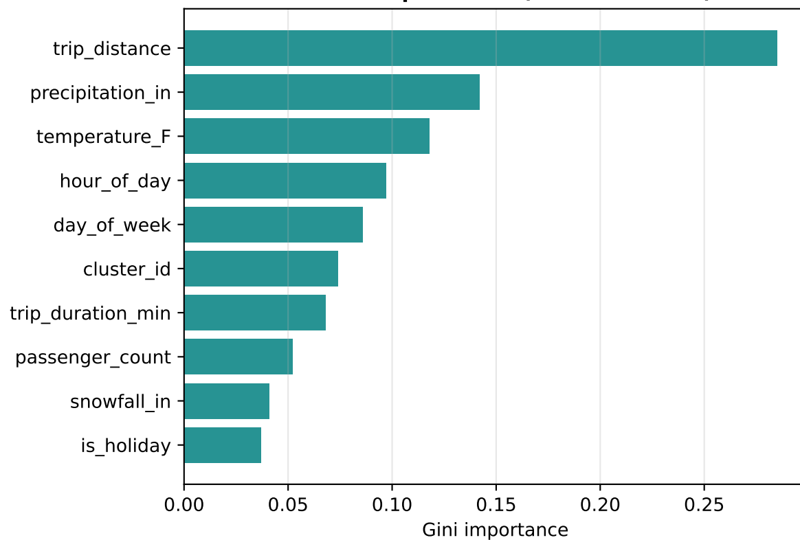
Feature Importances (Random Forest)
