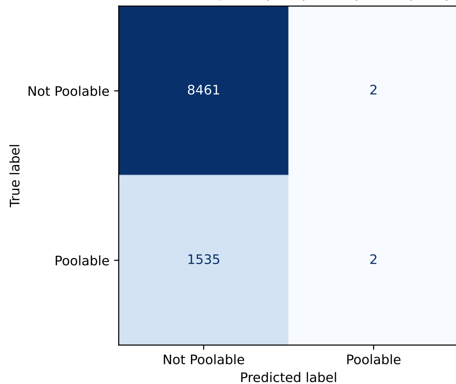
Confusion Matrix (TN=8,461, FP=2, FN=1,535, TP=2)
