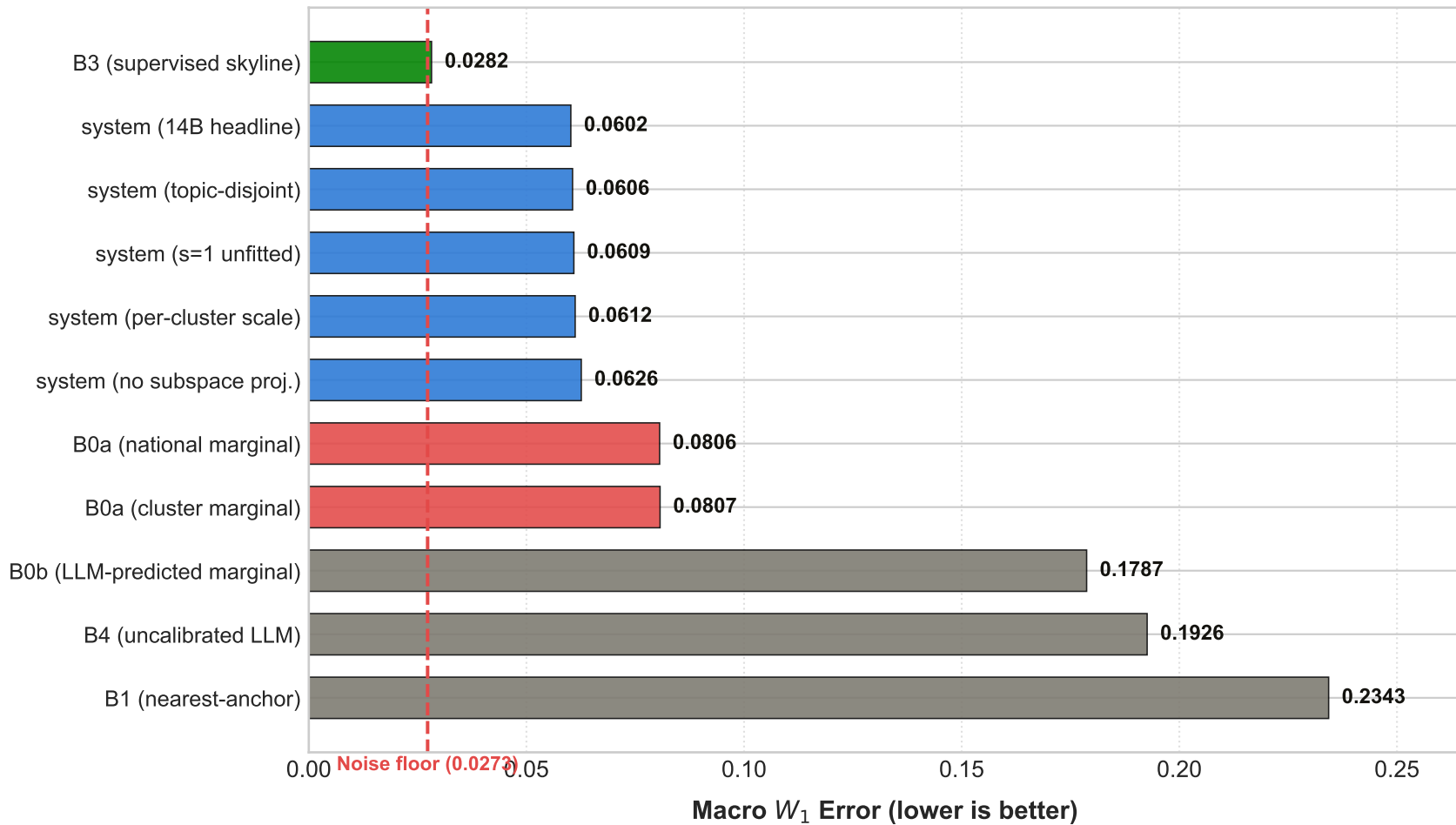
Macro W_1 Across All Arms (39 Scored Targets)
