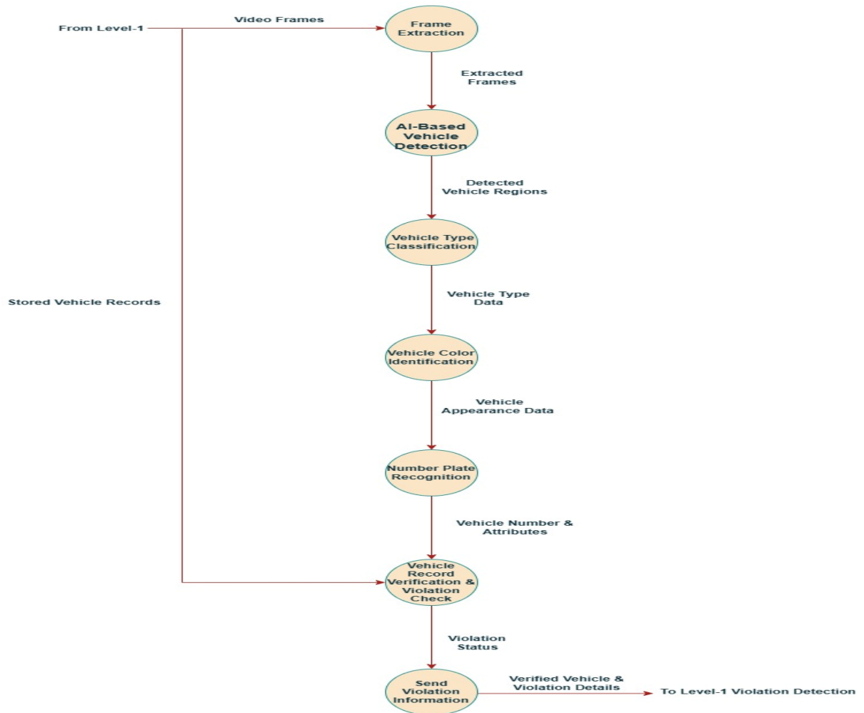
DFD Level-2 (Expansion of Vehicle Detection & Classification – Level-1 Process)
