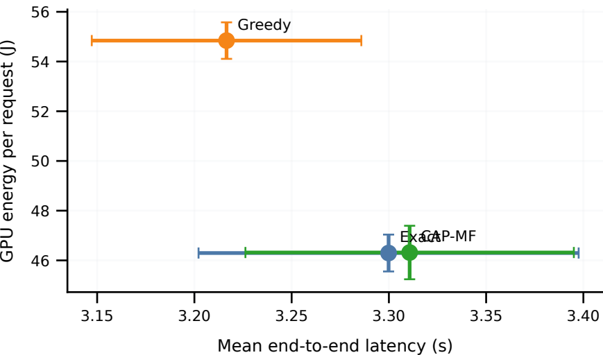
Five-repeat live vLLM energy-latency trade-off
