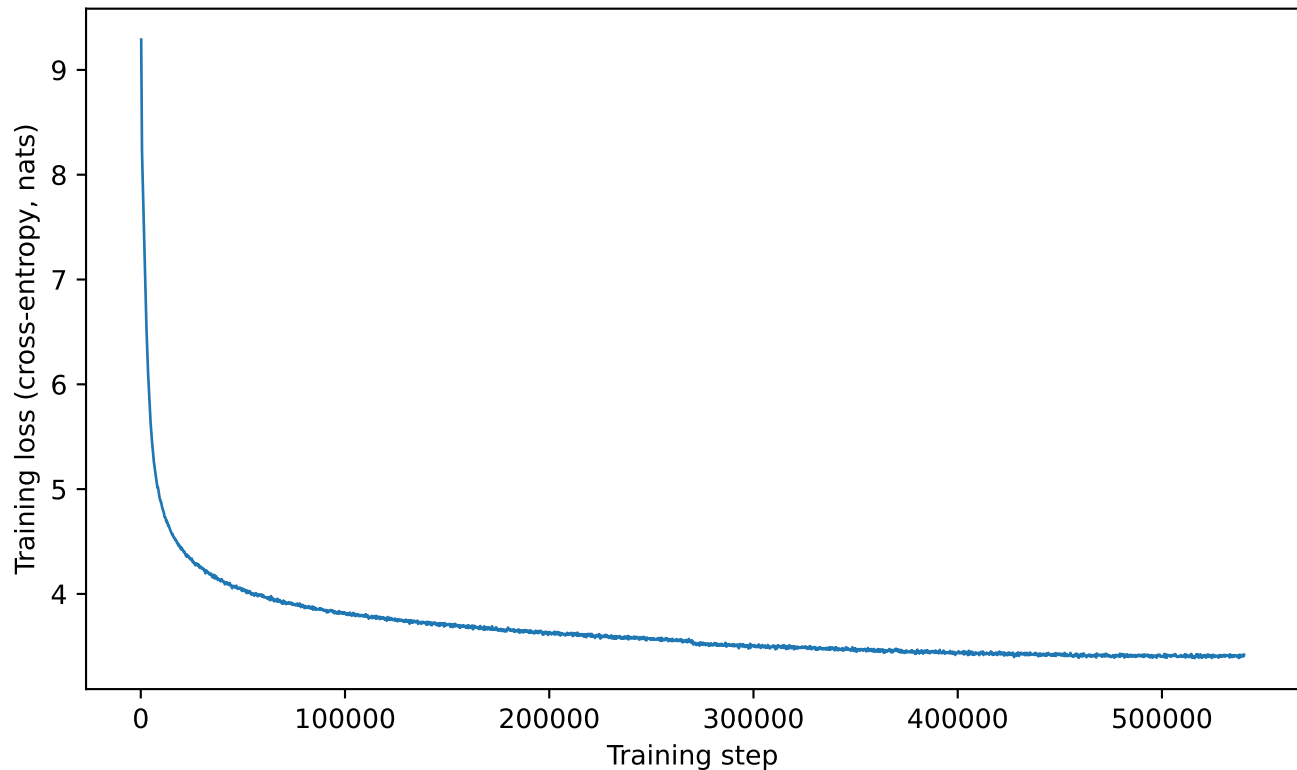
dravidian-gpt2-tamil: training loss
