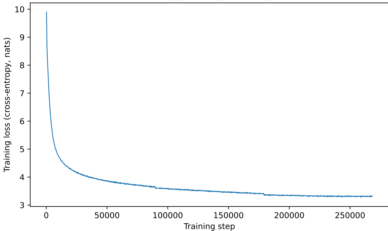
dravidian-gpt2-telugu: training loss
