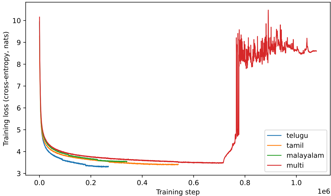
Pretraining loss
