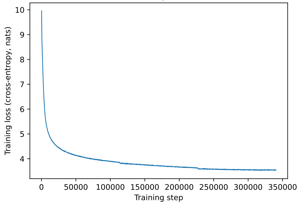
Training loss
