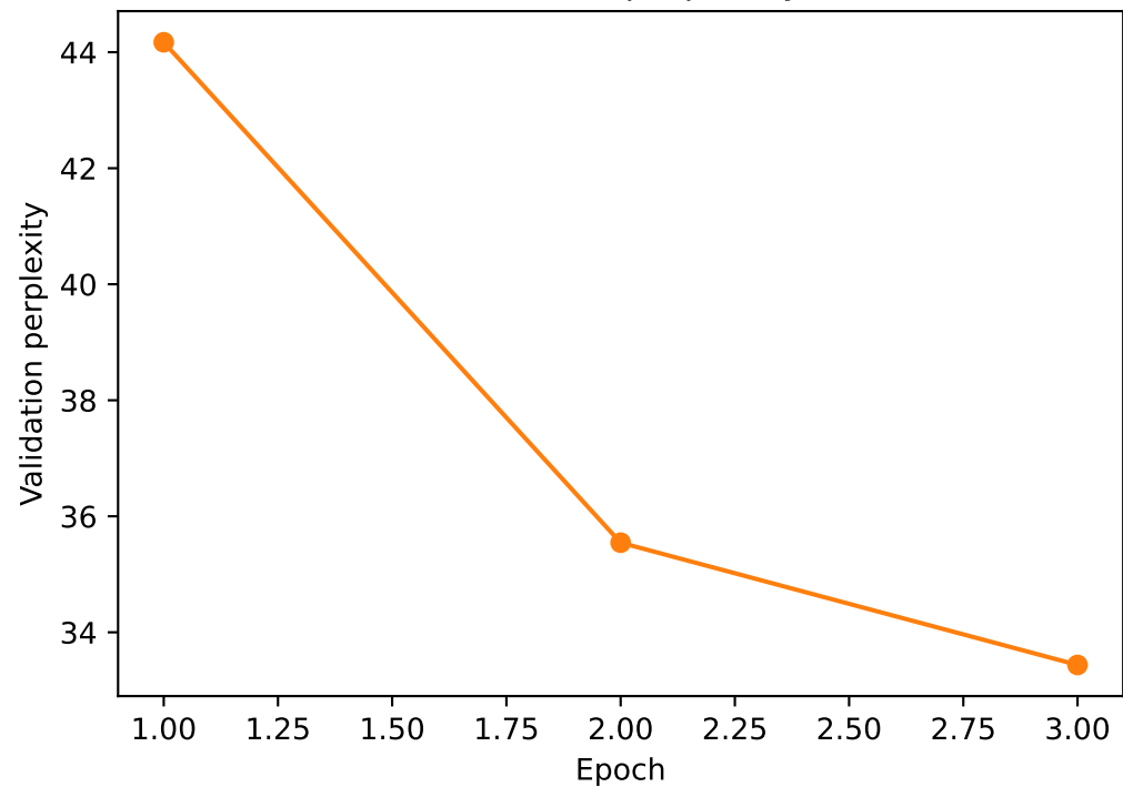
Validation perplexity
