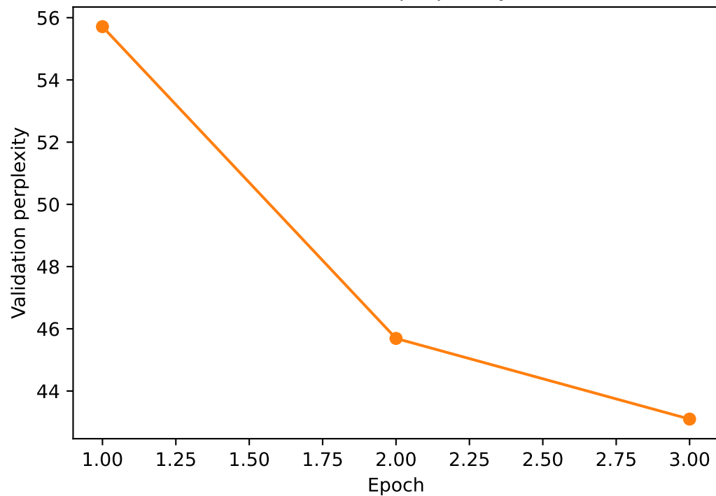
Validation perplexity
