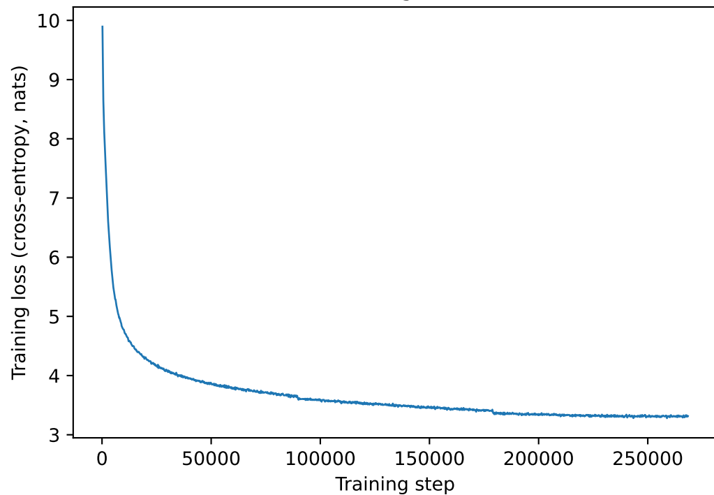
Training loss
