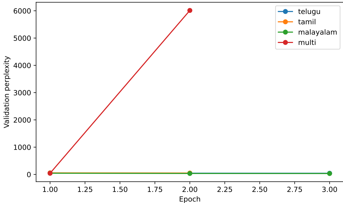
Validation perplexity across training
