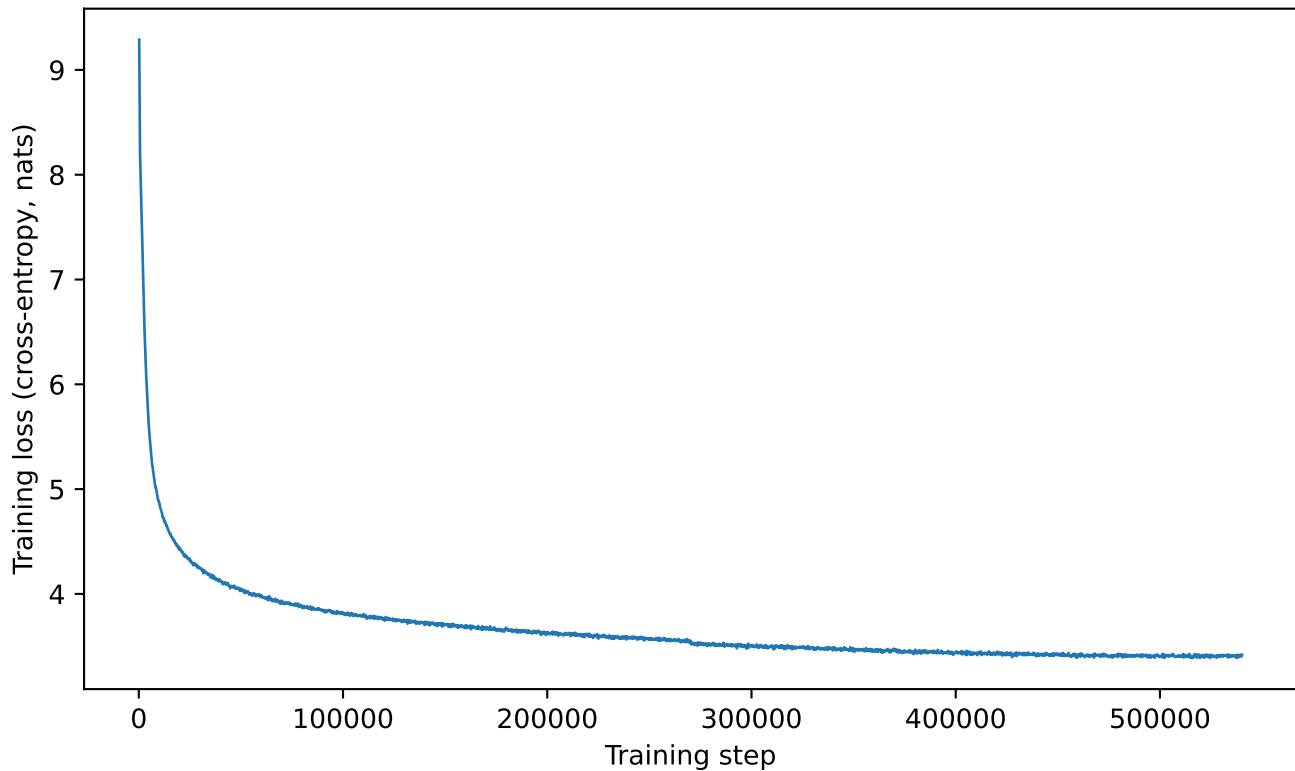
tamil-gpt2: training loss
