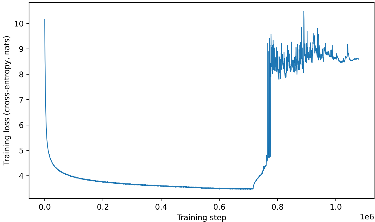
multi-gpt2: training loss
