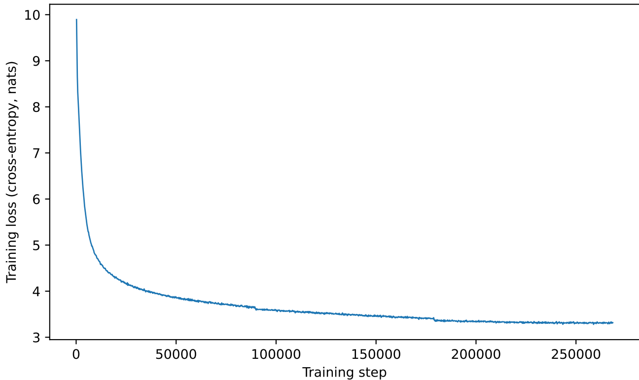
telugu-gpt2: training loss
