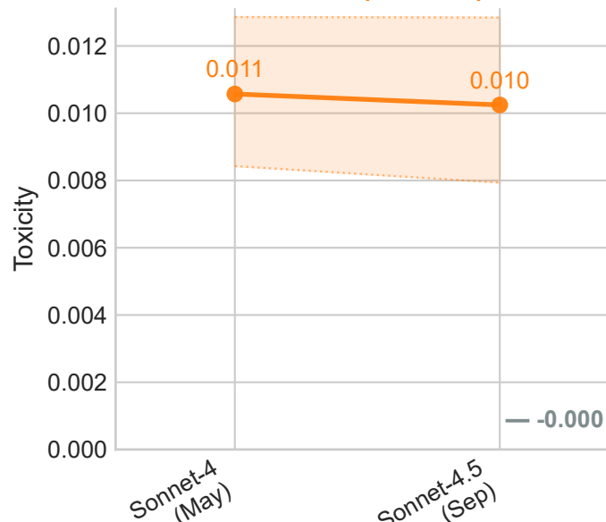
Claude (Sonnet)
