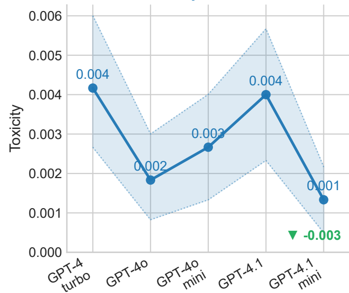
OpenAI
