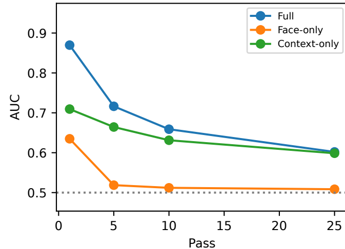
facefusion
