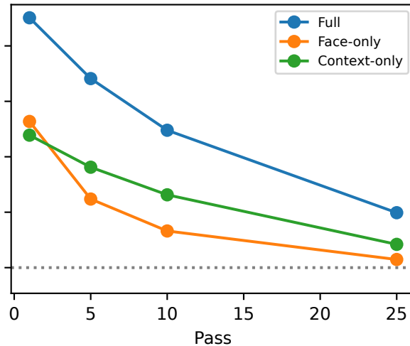
blendface
