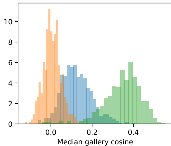
diffswap
