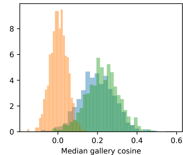
faceshifter
