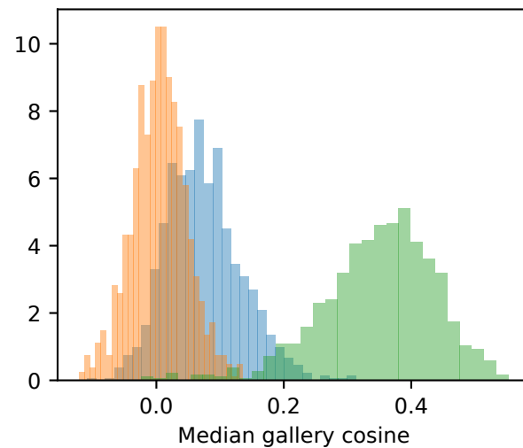
faceshifter
