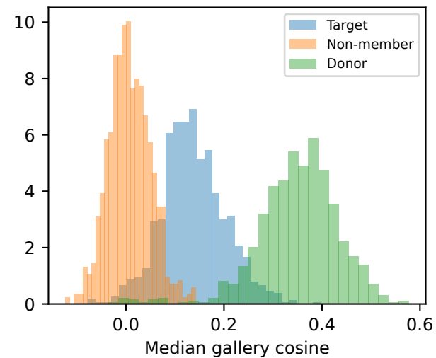
facefusion
