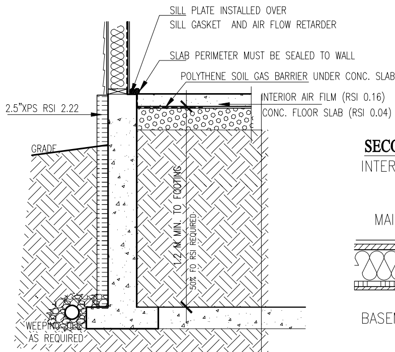
WALKOUT FOUNDATION&UNHEATED FLOOR (ABOVE FROST LINE-RSI 1.96 W/HRV) APPENDIX 9.34.2.8.(4)
