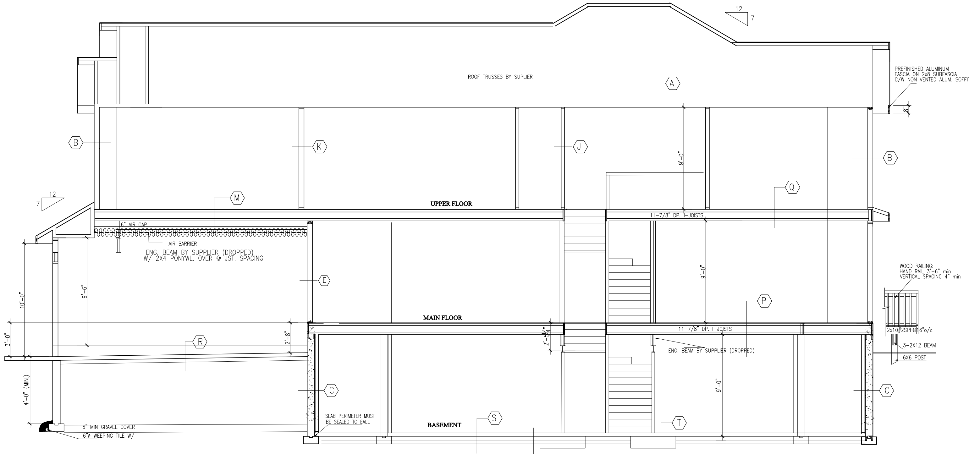
Cross Section (typ.) SCALE 3/16"=1'-0"
