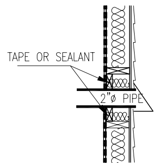
SERVICE PENITRATION IN EXTERIOR WALL DETAIL
