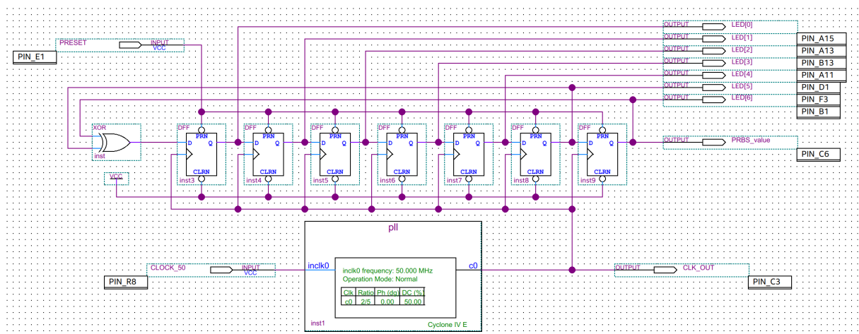
Figure 21: PRBS Generator implemented with 20MHz clock
