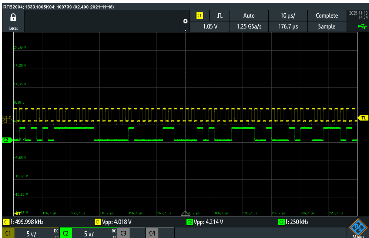
Figure 10: Oscilloscope capture of PRBS generator at 500kHz. First 7 bits in the figure are the 121 st -127 th bits of the sequence. Sequence repeats after
