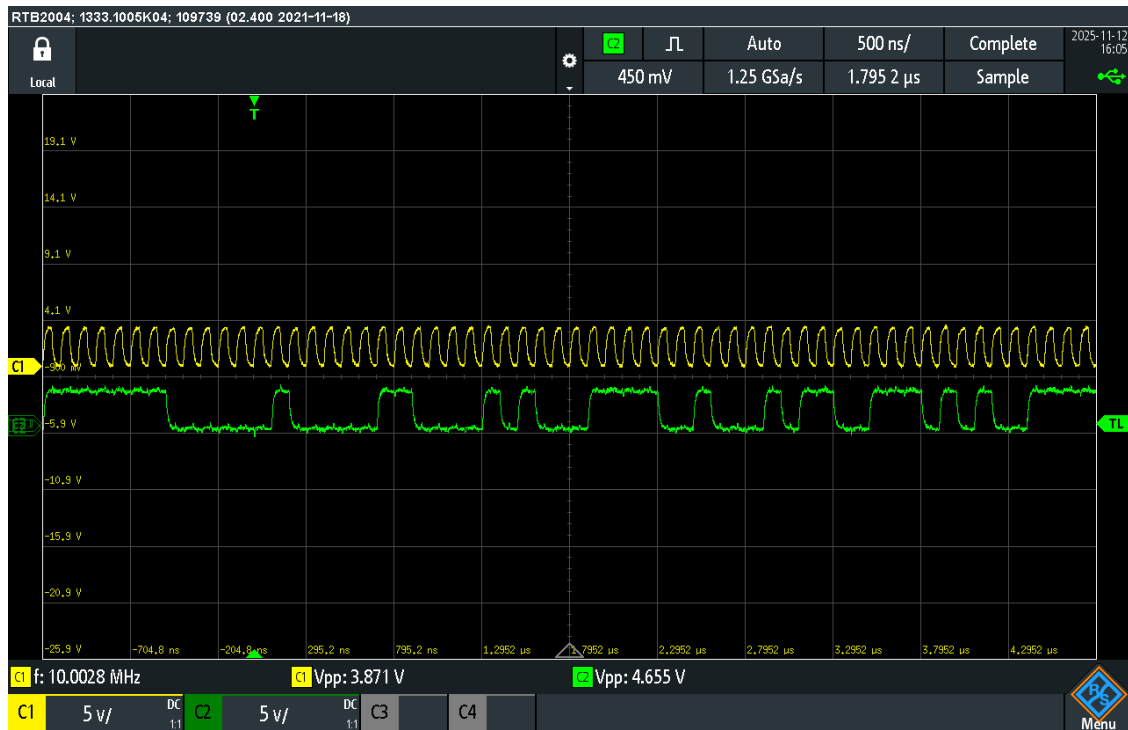
Figure 10: Oscilloscope output of PRBS generator at 10MHz (first 60 bits)
