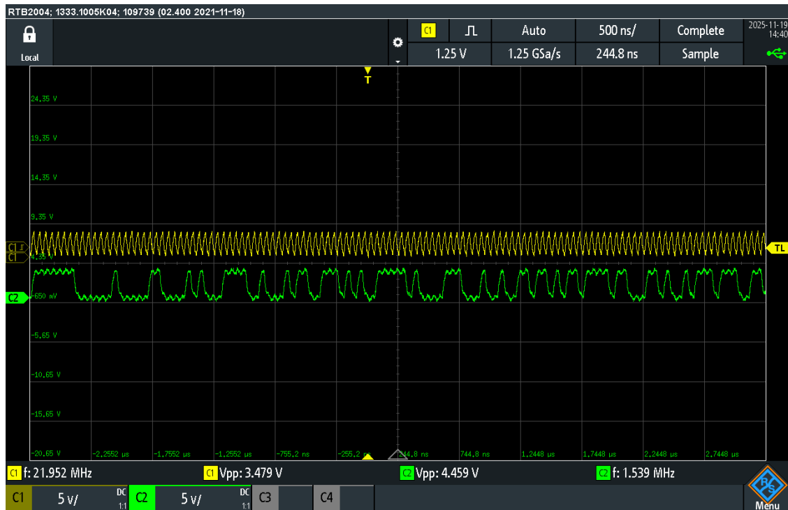
Figure 13: Oscilloscope output of PRBS generator at 20MHz (first 120 bits)
