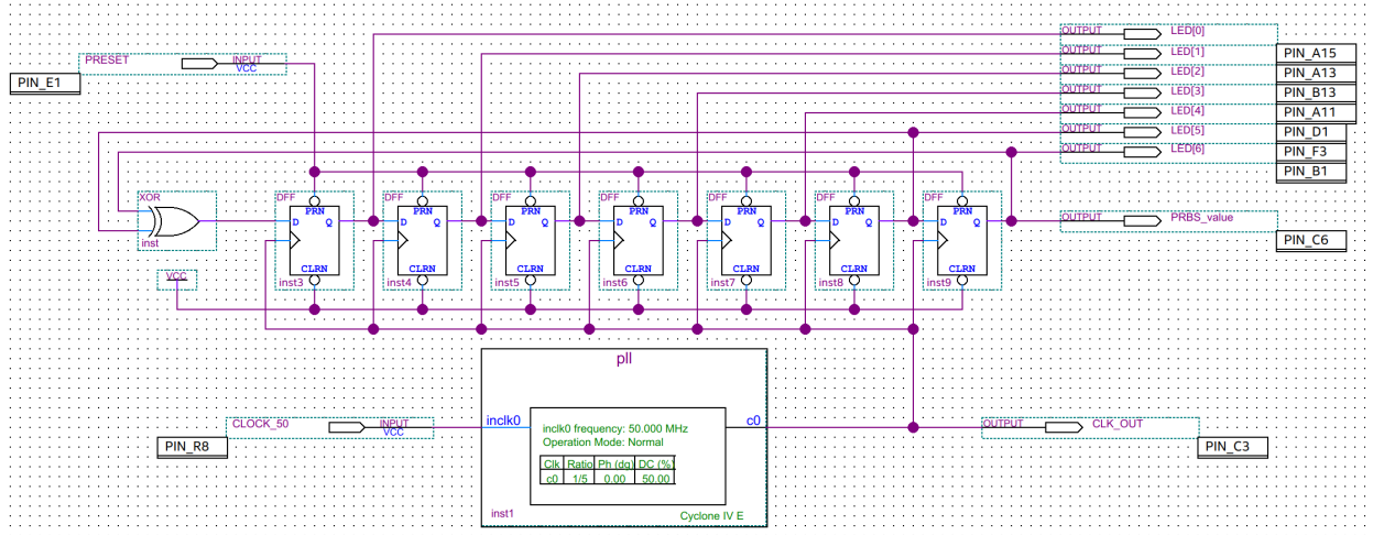
Figure 19: PRBS Generator implemented on Quartus Prime Lite with a 10MHz clock signal
