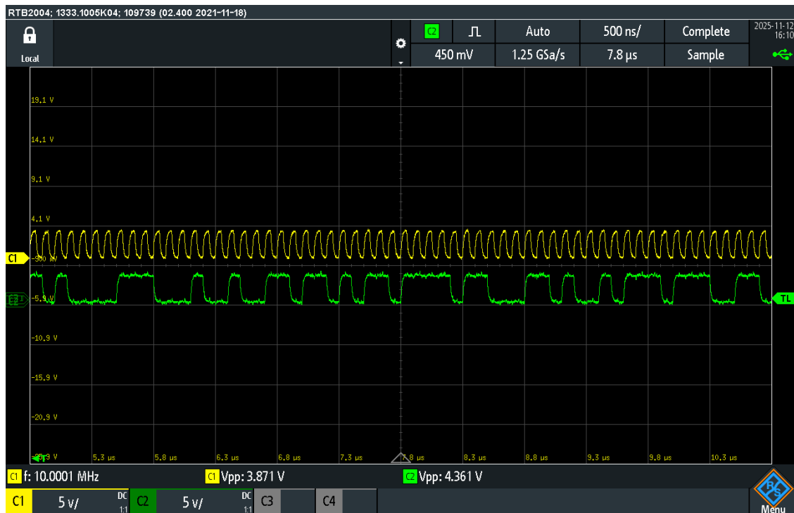
Figure 11: Oscilloscope output of PRBS generator at 10MHz (61st to 120th bits)
