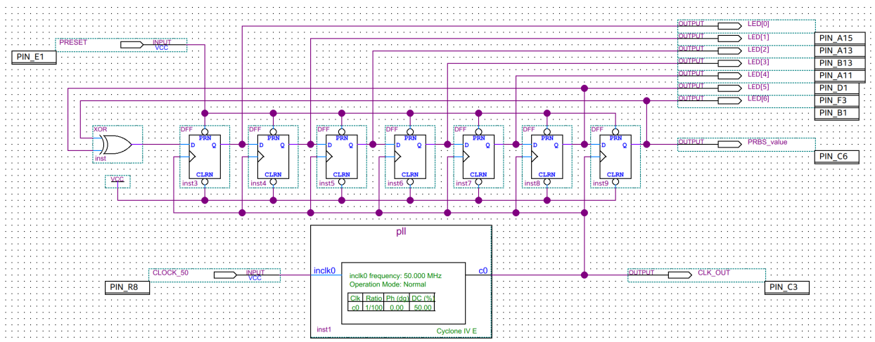
Figure 18: PRBS Generator implemented on Quartus Prime Lite with a 500kHz clock signal
