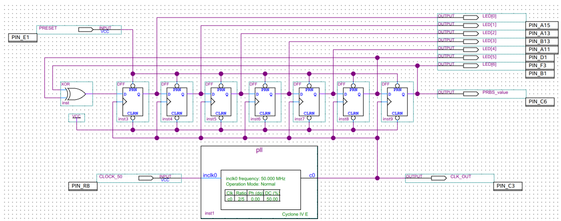
Figure 20: PRBS Generator implemented on Quartus Prime Lite with a 20MHz clock signal
