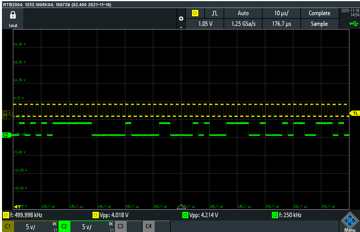
Figure 9: Oscilloscope output of PRBS generator at 500kHz. First 7 bits in the figure are the 121st to 127th bits of the sequence. Sequence repeats after this
