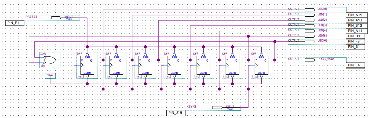
Figure 17: PRBS Generator implemented on Quartus Prime Lite with the clock tied to a push button
