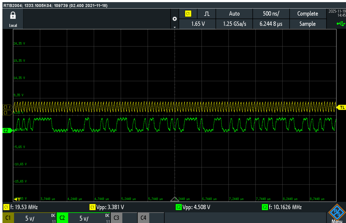
Figure 14: Oscilloscope output of PRBS generator at 20MHz First 7 bits in the figure are the 121st to 127th bits of the sequence. Sequence repeats after this
