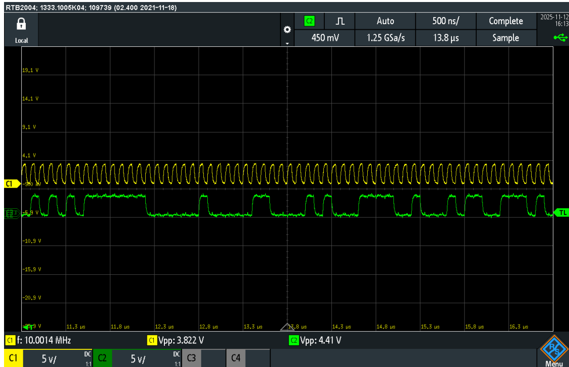
Figure 12: Oscilloscope output of PRBS generator at 10MHz. First 7 bits in the figure are the 121st to 127th bits of the sequence. Sequence repeats after this
