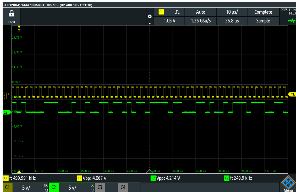
Figure 8: Oscilloscope output of PRBS generator at 500kHz (61st to 120th bits)
