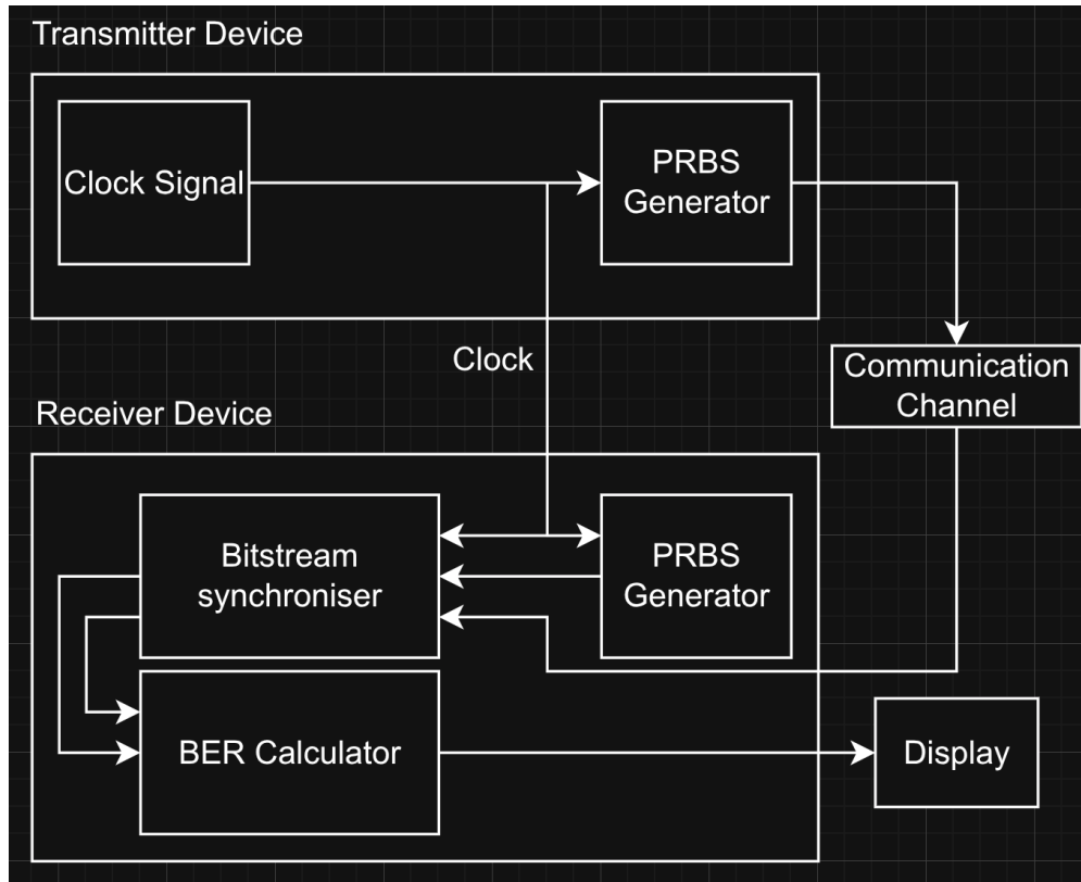
Figure 1: Block Diagram of BER Testing system
