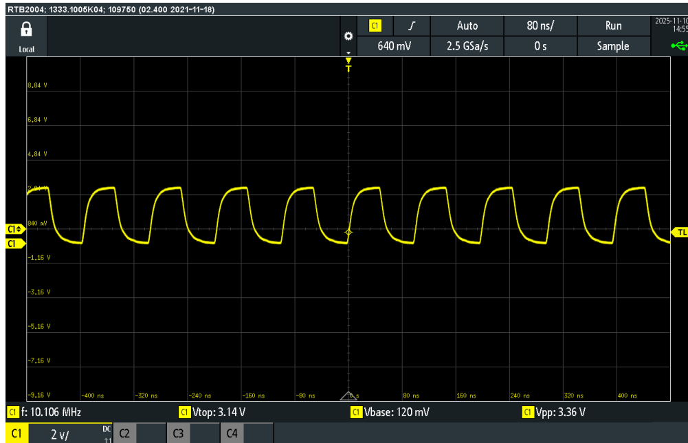
Figure 2: Oscilloscope capture of 10MHz clock from NUCLEO-F401RE
