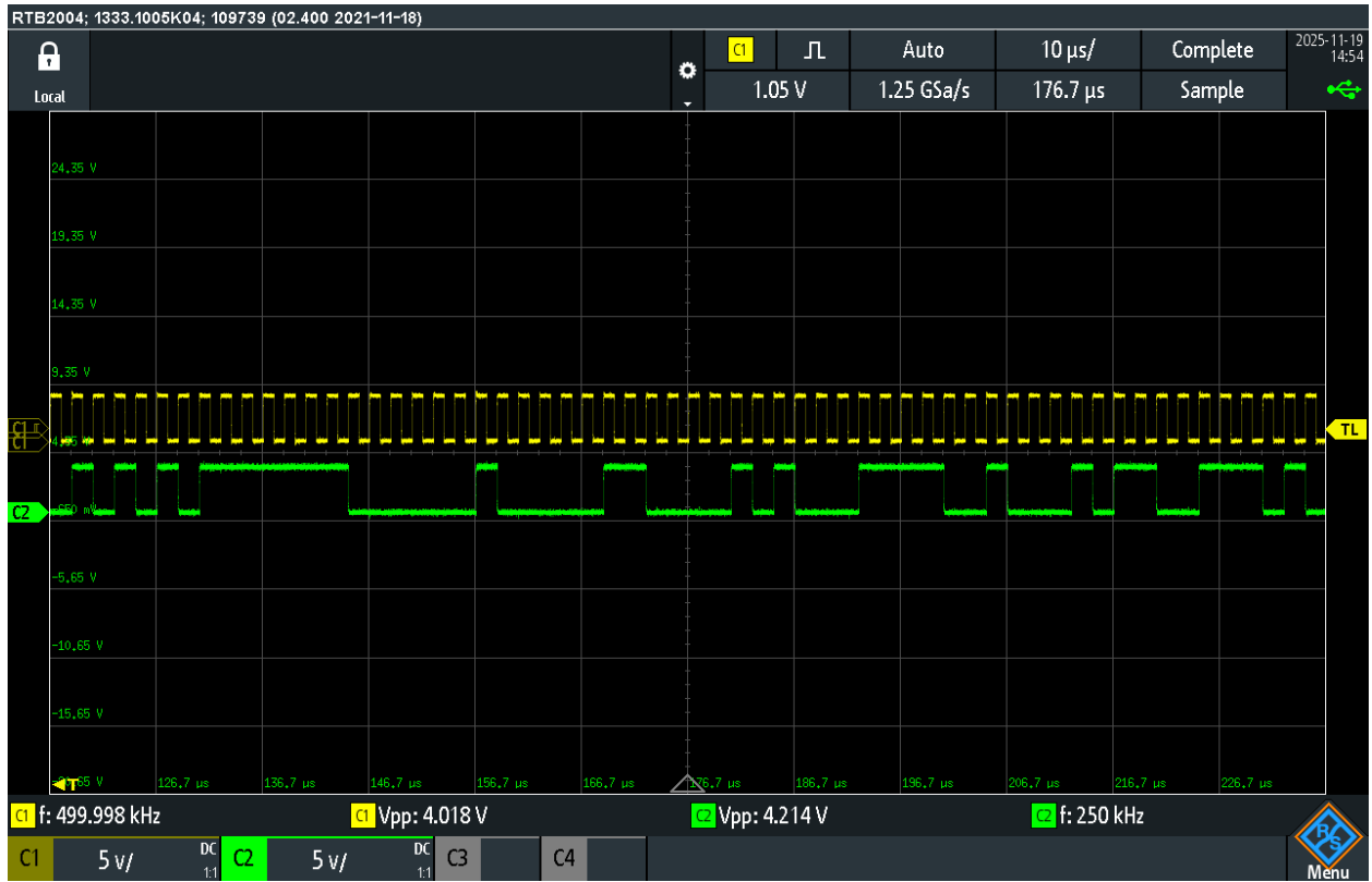
Figure 10: Oscilloscope output of PRBS generator at 500kHz. First 7 bits in the figure are the 121 st -127 th bits of the sequence. Sequence repeats after
