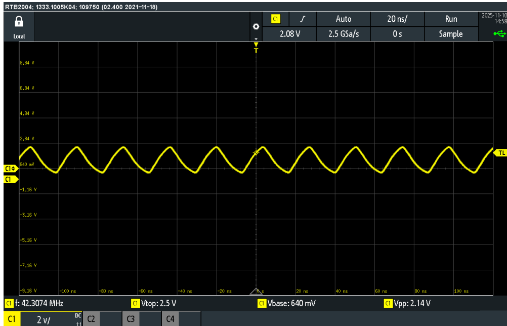
Figure 4: Oscilloscope capture of 42MHz clock from NUCLEO-F401RE
