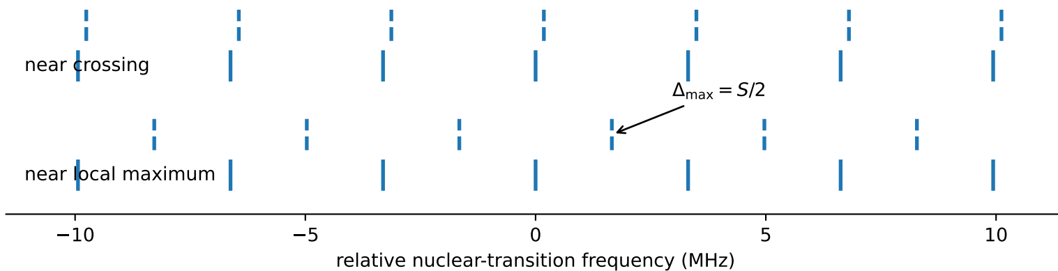
(a) Two electron-conditioned nuclear spectra are rigid combs
