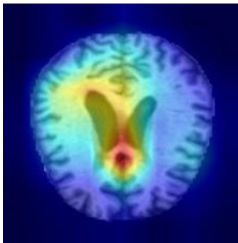
GradCAM Activation
