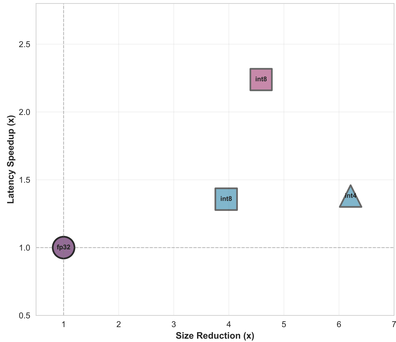
Model Optimization Performance Dashboard BERT QNLI Top-Right with Larger Bubbles = Best (High Compression + High Speed + High Accuracy) BERT SST2
