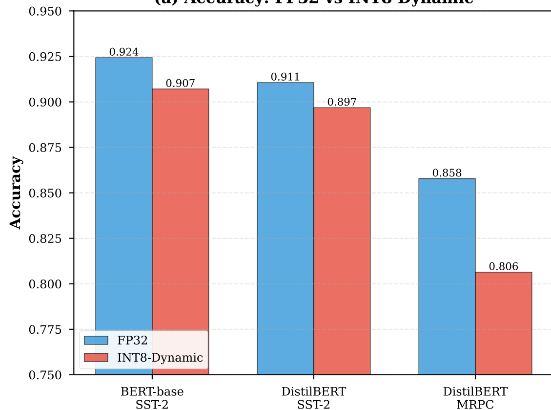
(a) Accuracy: FP32 vs INT8 Dynamic
