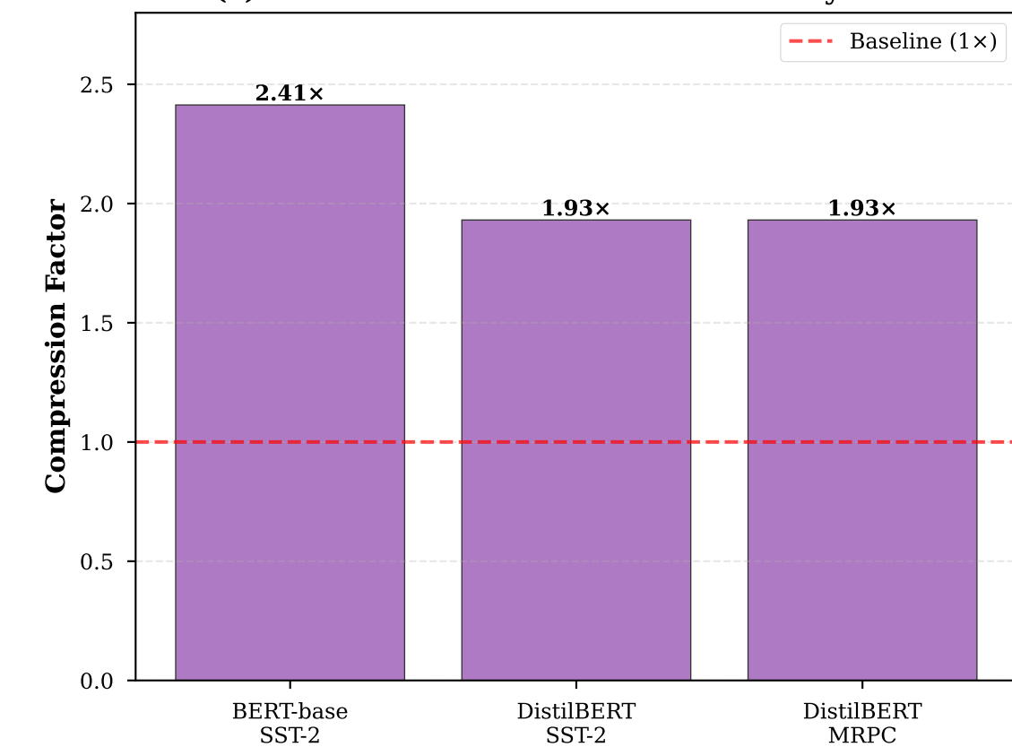
(c) Model Size Reduction with INT8 Dynamic
